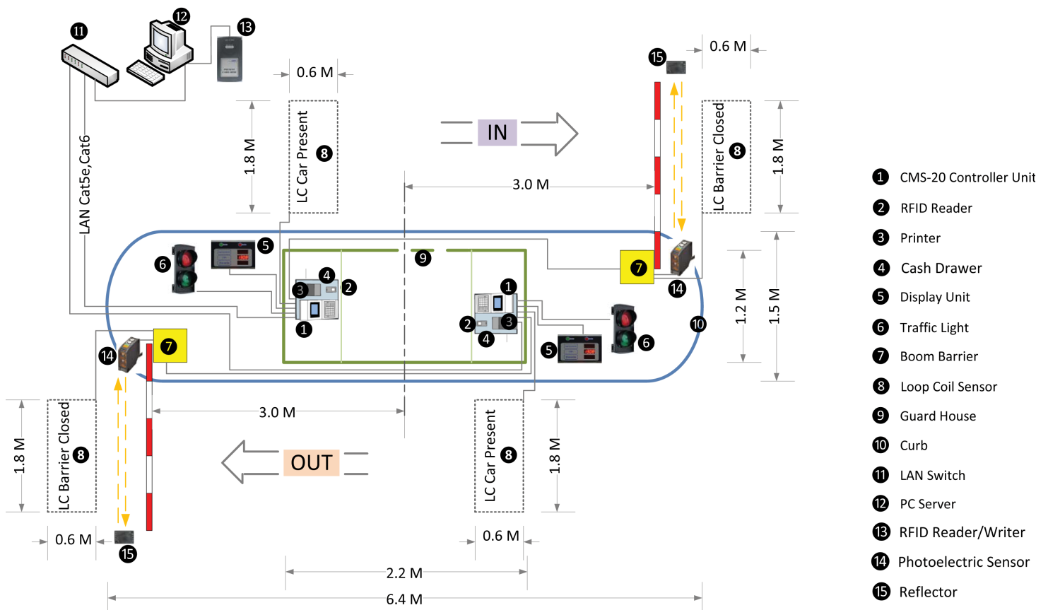
Carpark Diagram
